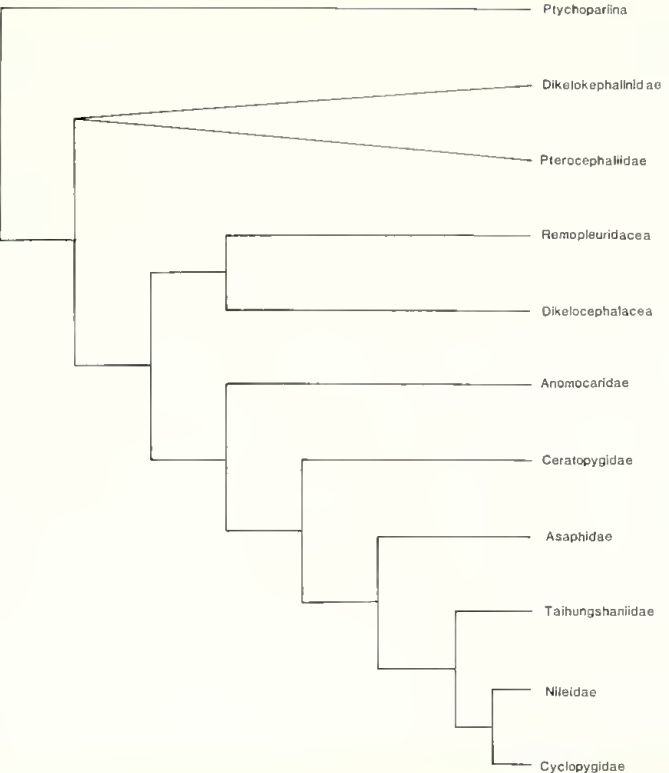
TEXT-FIG. 4. Consensus tree derived from text-figs. 2 and 3, according to the method of Adams (1972). Characters not included.
